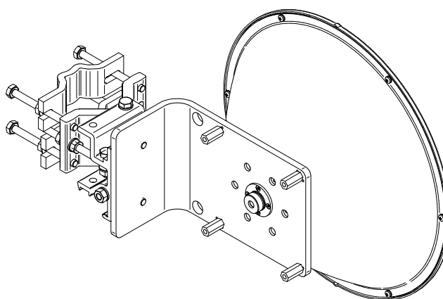
Fig. 2 Antenna with massive bracket (back side)
